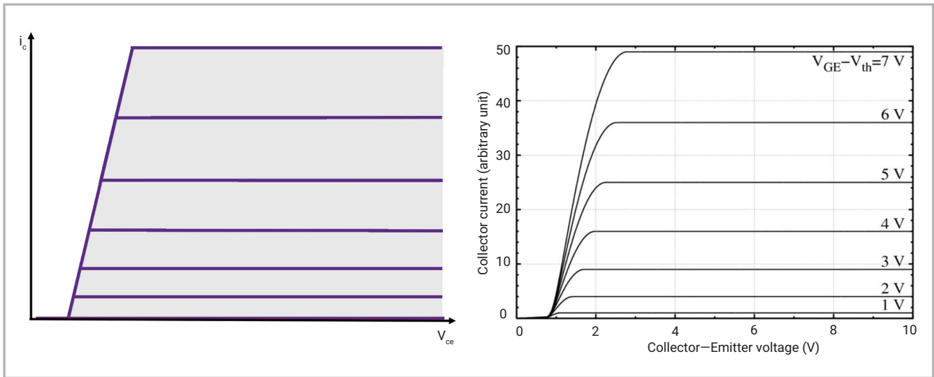
Figure 4: Comparison of PWL and SPICE-level models
