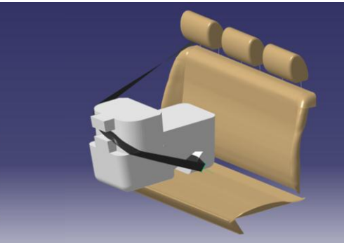
Fig. 4: Safe belt system for children using Gabarit test devices
